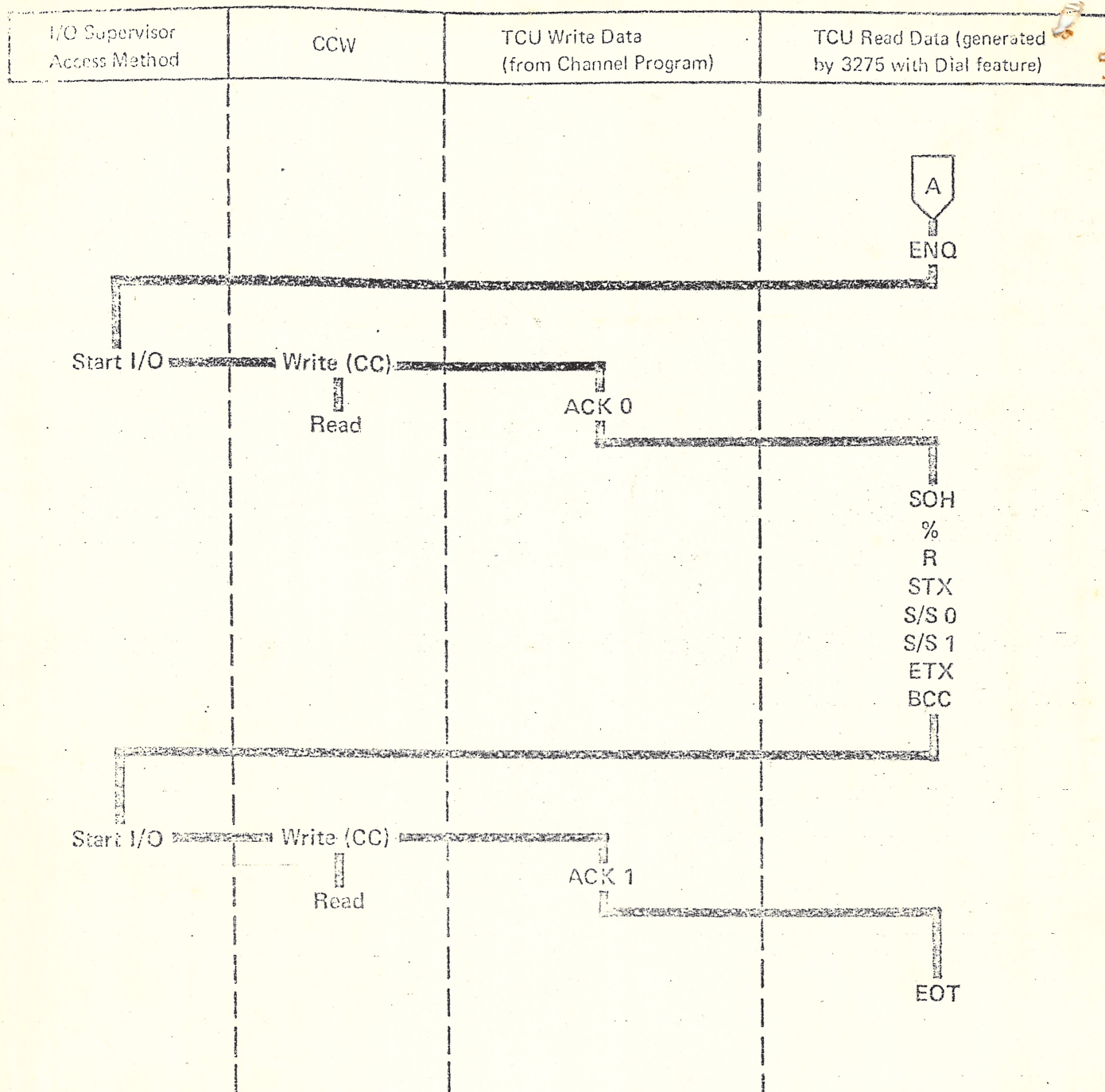
Figure 6-13 Status Message Transmission with Dial Feature, Sequence/Response Diagram
