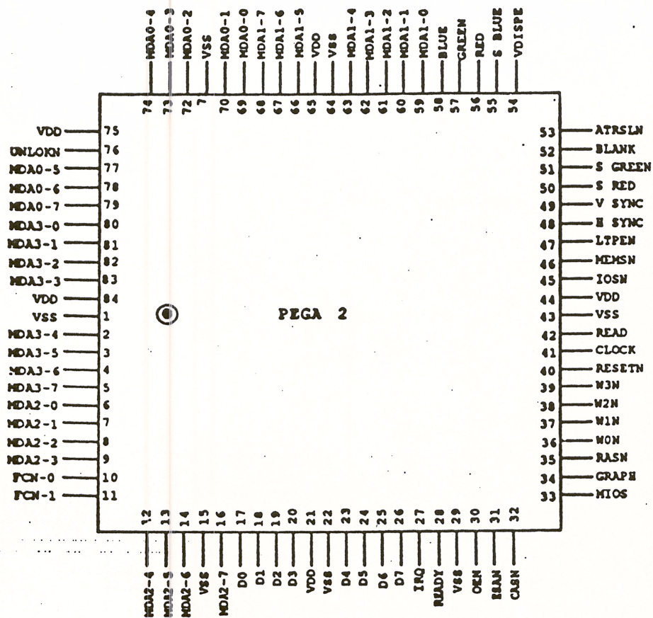
Figure 2 : 84 - Pin Plastic Leaded Chip Carrier
