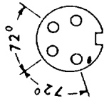
DIN 4 pin Fully Screened Line Socket. 2004
